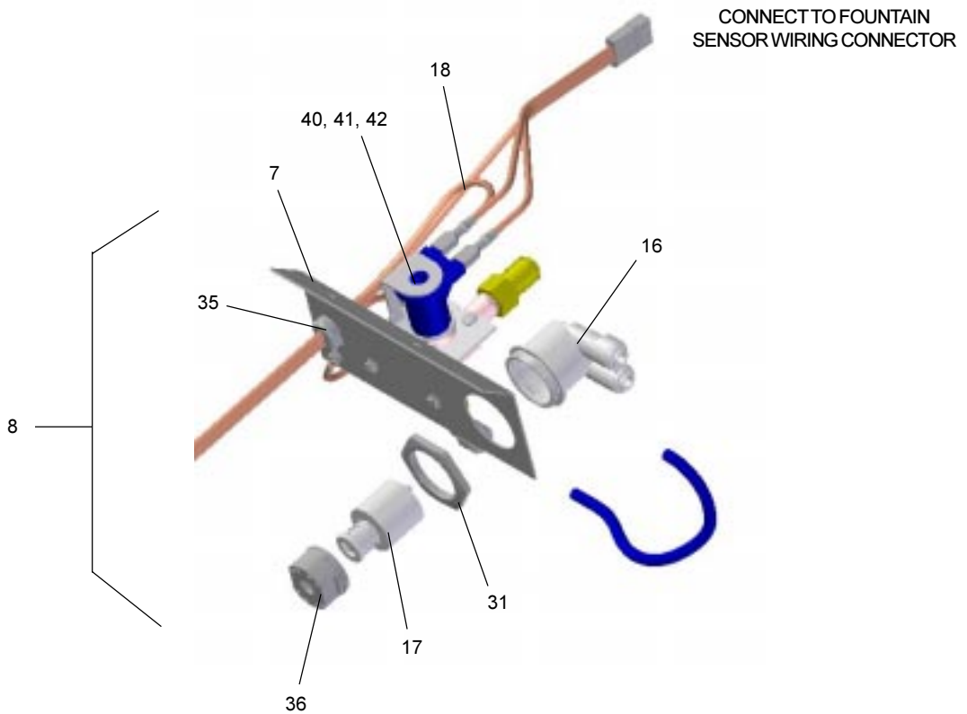
Figure 8 - Regulator Assembly
