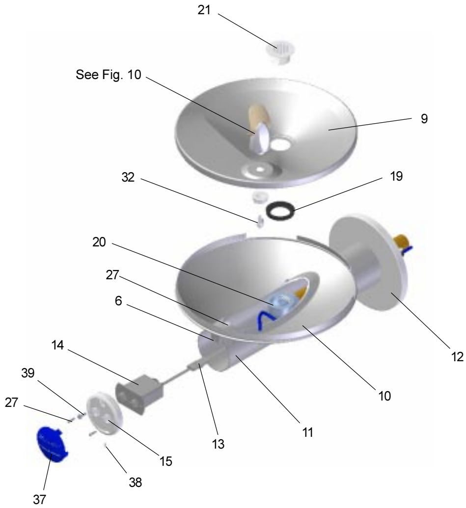
Figure 9 - Exploded View
