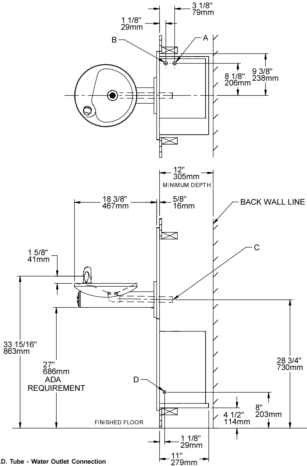
Figure 1 - Rough-in Dimensions
