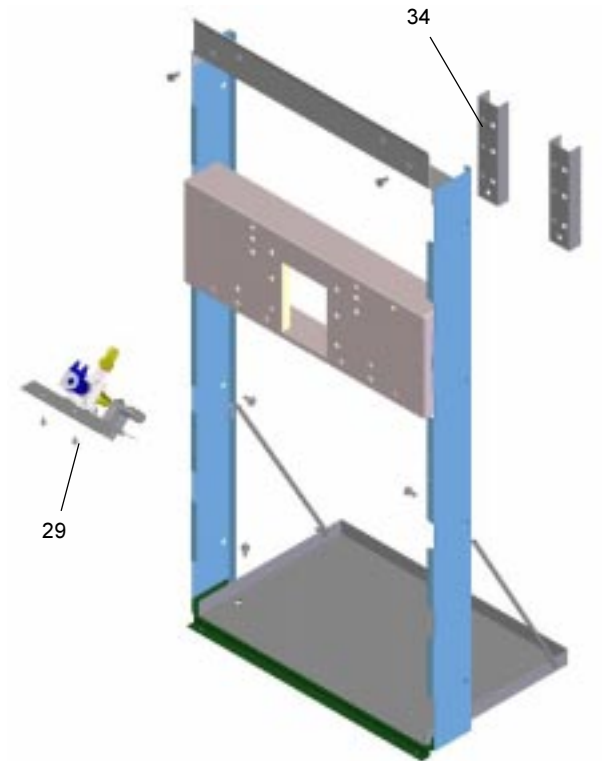
Figure 7 - Solenoid Assembly
