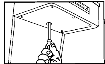
Cartridge flow adjustment through bottom panel. Clockwise increases flow.
